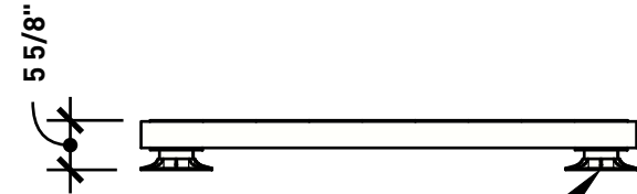
ScrewJack Deck Support Pedestals
